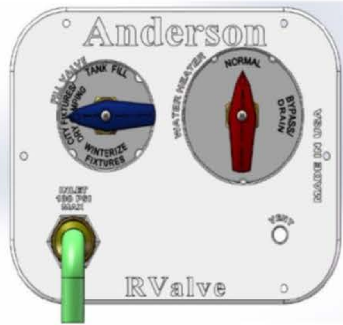
Normal use (pressurized water source)
