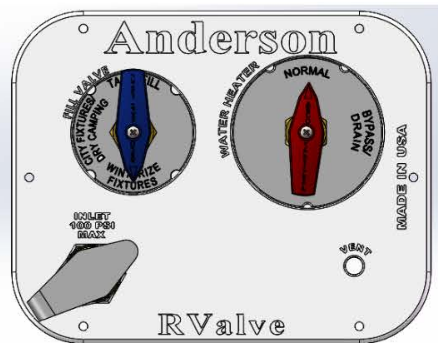
Filling the fresh water tank and water heater (gravity fill)
