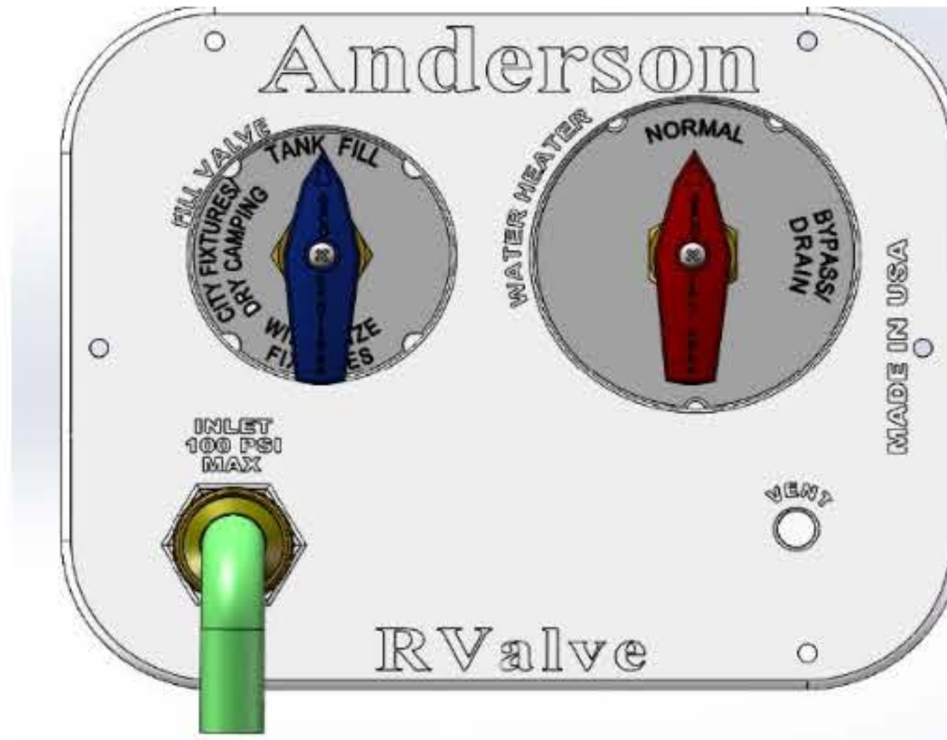
Filling the fresh water tank (pressurized water source)
